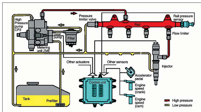
"COMMON RAIL" DOOSAN DLo6 ENGINE
