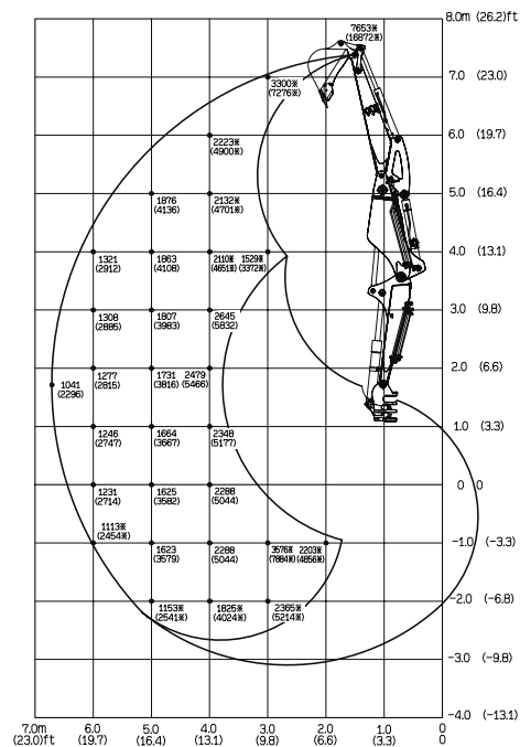
Over Front ; Dozer Blade Up
