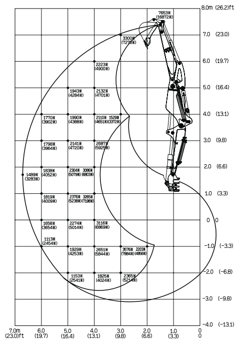
Over Front ; Dozer Blade Down
